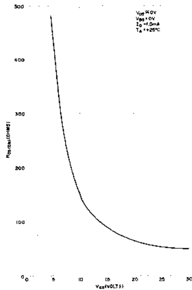
DRAIN TO SOURCE RESISTANCE vs GATE VOLTAGE
