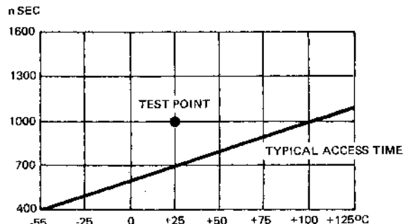
ACCESS TIME VS. TEMPERATURE
