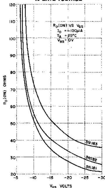
DRAIN TO SOURCE RESISTANCE vs GATE VOLTAGE
