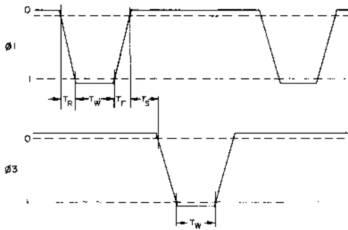
Fig.1 CLOCK WAVEFORMS
