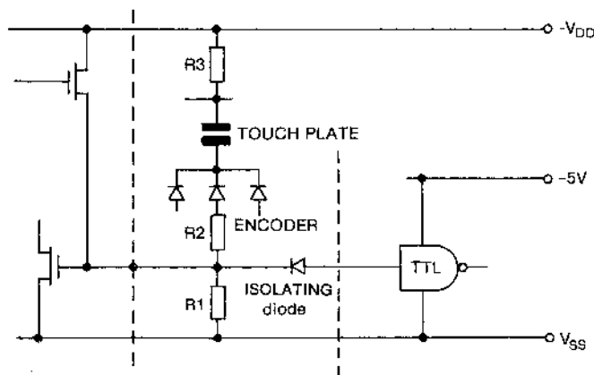
Fig.1 INPUT/OUTPUT CIRCUIT
