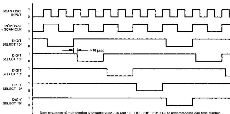
Fig.3 SCAN CLOCK INPUT AND MULTIPLEXING DIGIT SELECT OUTPUT
