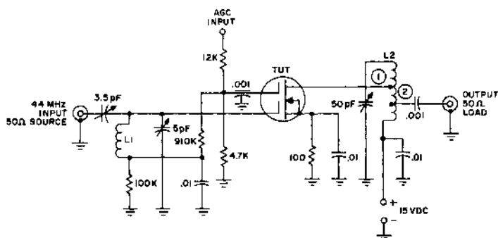
Fig. 3 — 44MHz POWER GAIN/NOISE FIGURE TEST CIRCUIT
