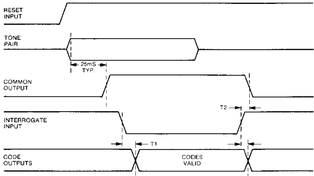
Fig.1 "HANDSHAKING" TIMING DIAGRAM
