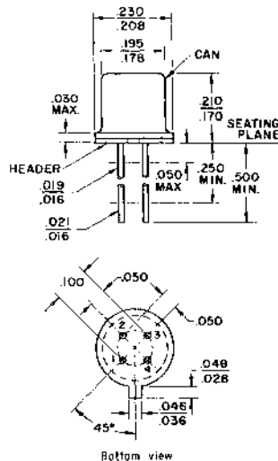
TO-72
