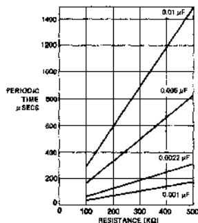
Fig. 3 OSCILLATOR CHARACTERISTICS FOR V_p = 10V
