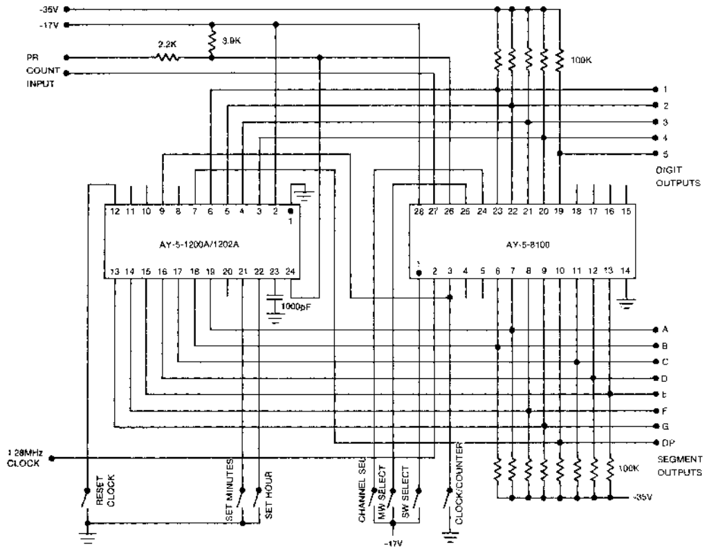
Fig.2 FREQUENCY COUNTER/CLOCK CONNECTION DIAGRAM-DIRECT FLORESCENT DISPLAY DRIVE
