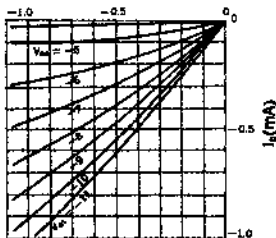
DRAIN CHARACTERISTICS AT 25°C V_{GS} (VOLTS)
