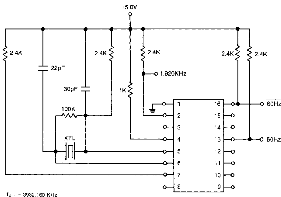
Fig. 4 — TYPICAL APPLICATION (60Hz CLOCK)
