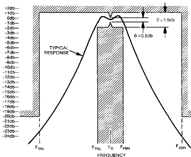
Fig.1 FREQUENCY RESPONSE
