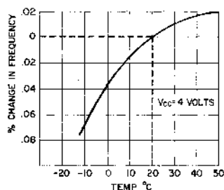
Fig.2. OSCILLATOR CHARACTERISTICS
