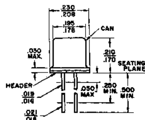
TO-72
