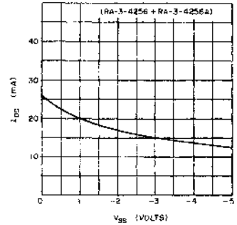
TYPICAL I_{OD} VS. V_{SS} (for memory hold during power down)
