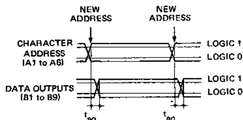
Fig. 3 ADDRESS TO OUTPUT DELAY TIME
