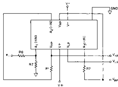
Fig. 3 NON-INVERTING CONFIGURATION
