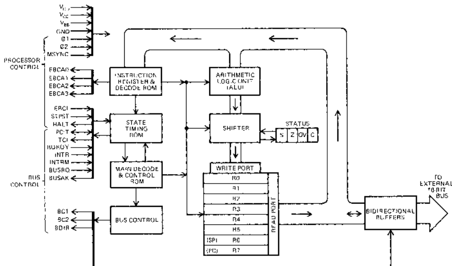
CP1600 INTERNAL BLOCK DIAGRAM
