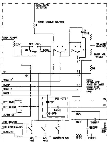
Fig.15 RADIO SWITCHING
