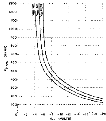
DRAIN TO SOURCE RESISTANCE vs. GATE VOLTAGE
