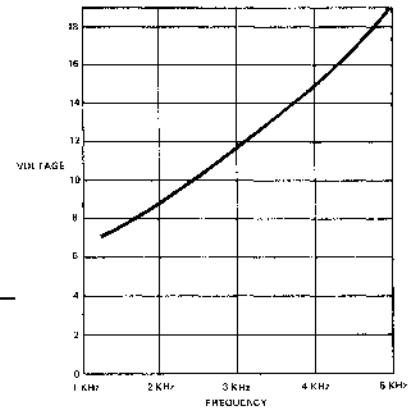
Fig. 4 OSCILLATOR FREQUENCY VS. SUPPLY VOLTAGE ( V_p ) R=680K C=2000\text{ pf}
