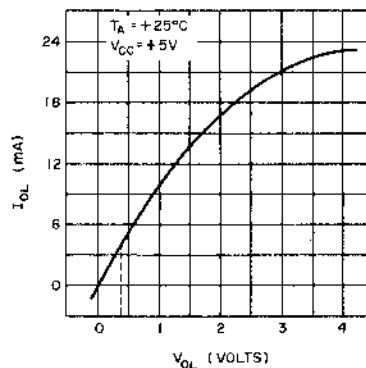
Fig.5 OUTPUT SINK CURRENT VS. OUTPUT VOLTAGE
