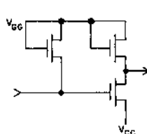
Fig.5 TRUE/COMPLEMENT INPUT
