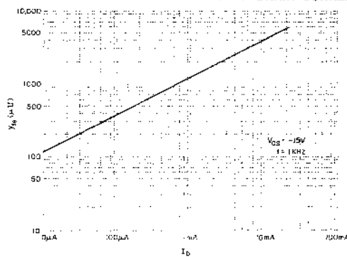
FORWARD TRANSCONDUCTANCE vs. DRAIN CURRENT
