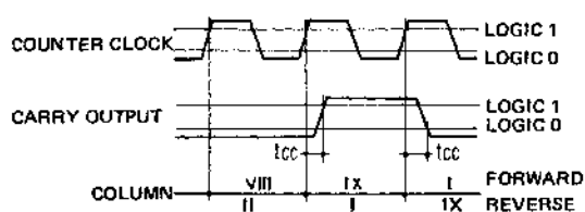
Fig. 8 CLOCK TO CARRY DELAY TIME
