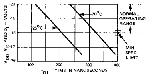
Fig. 1 TYPICAL \phi_1 DELAY IN NANoseconds vs. POWER SUPPLY VOLTAGE (ER2800)
