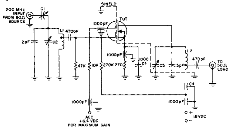
Fig. 1 — 200MHz POWER GAIN/NOISE FIGURE TEST CIRCUIT
