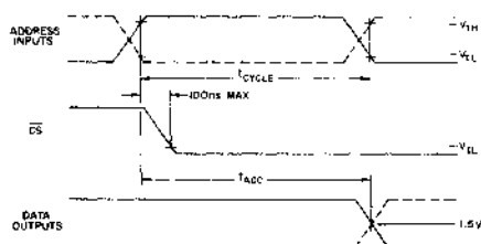
READ ACCESS
