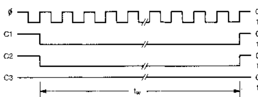
Fig.6 WRITE
