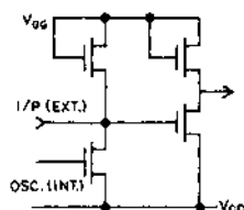
Fig.3 DIGIT SELECT CLOCK INPUT
