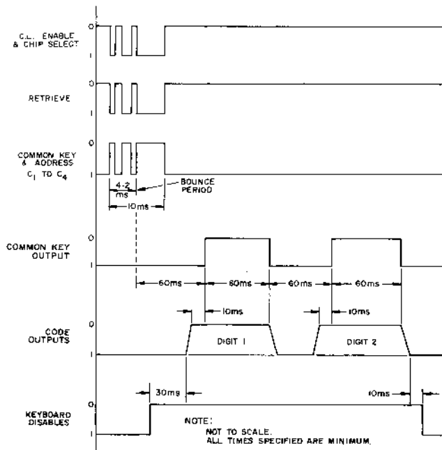
Fig.3 "RETRIEVE" WAVEFORMS
