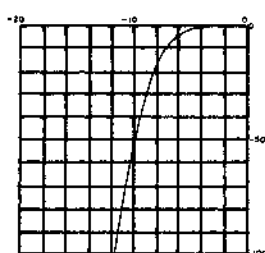
TURN-ON CHARACTERISTICS AT 25°C V_{GS} = V_{DS} (VOLTS)
