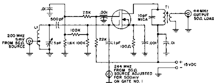
FIG. 2 — 200MHz TO 44MHz MIXER TEST CIRCUIT
