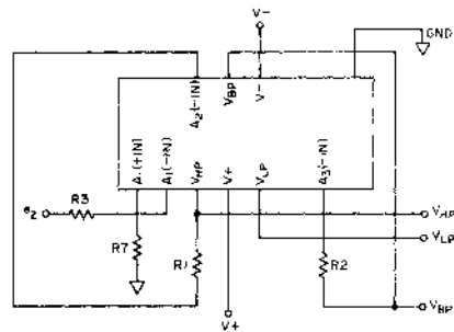
Fig. 4 INVERTING CONFIGURATION
