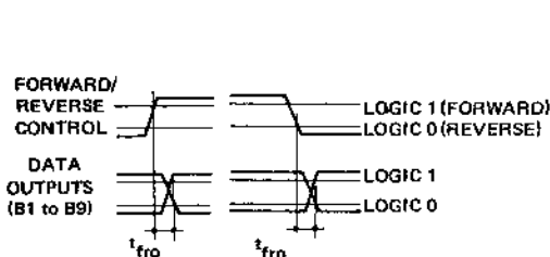
Fig. 5 FORWARD/REVERSE TO OUTPUT DELAY TIME
