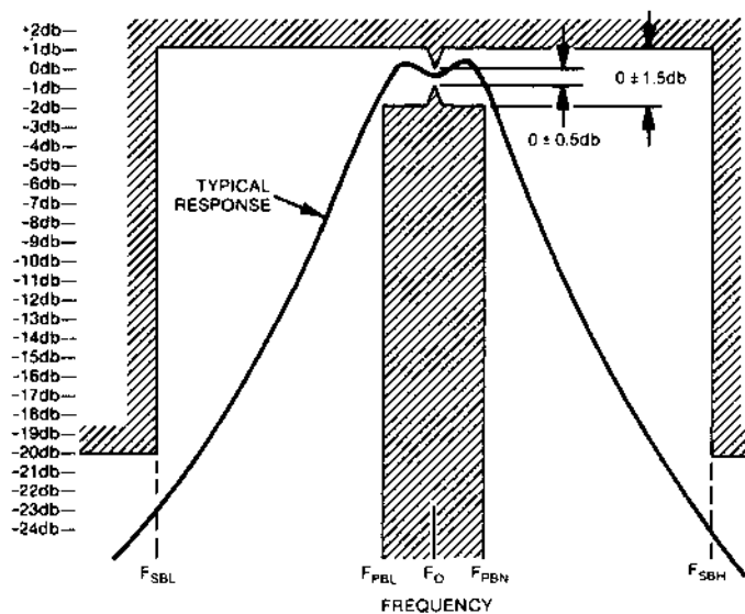
Fig.1 FREQUENCY RESPONSE
