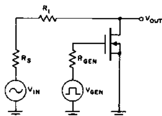
SHUNT CHOPPER
