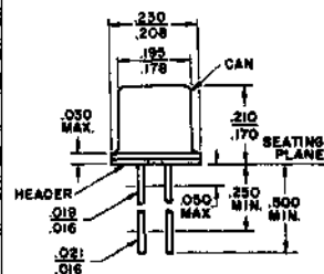
TO-72
