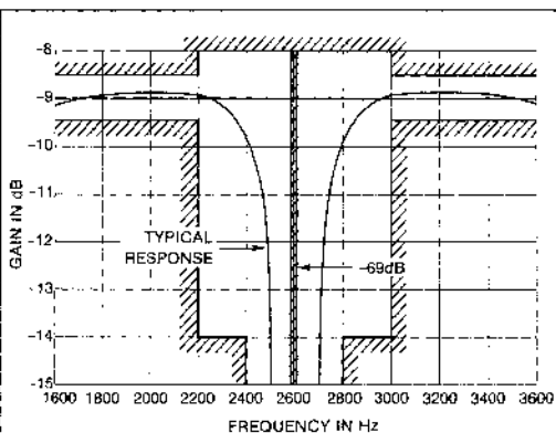
Fig. 1 FREQUENCY RESPONSE LIMITS ACF 7410C
