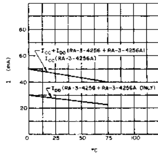
TYPICAL POWER SUPPLY CURRENT VS. TEMPERATURE
