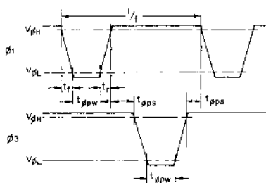
Fig.1 Clock Waveforms
