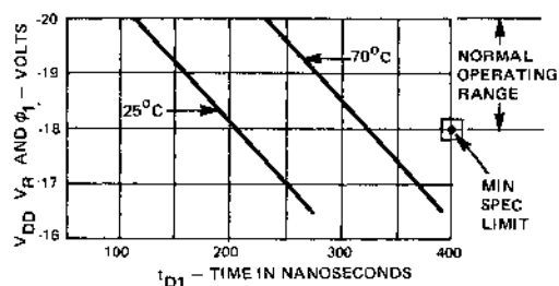
Fig.1 TYPICAL \phi1 DELAY IN NANOSECONDS VS. POWER SUPPLY VOLTAGE
