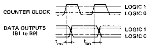
Fig. 4 CLOCK TO OUTPUT DELAY TIME
