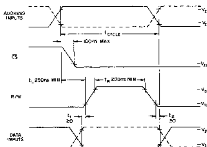
WRITE CYCLE
