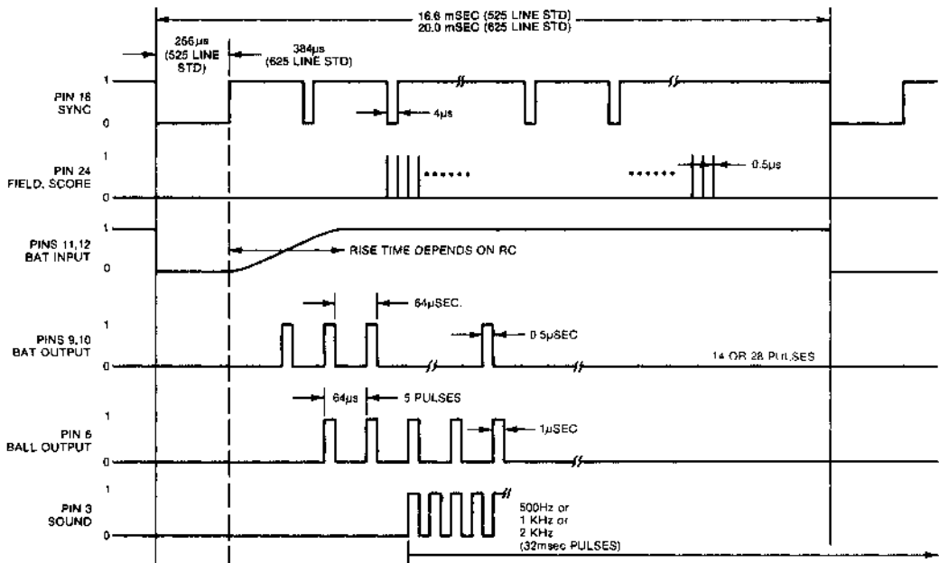
Fig.11 TIMING DIAGRAM
