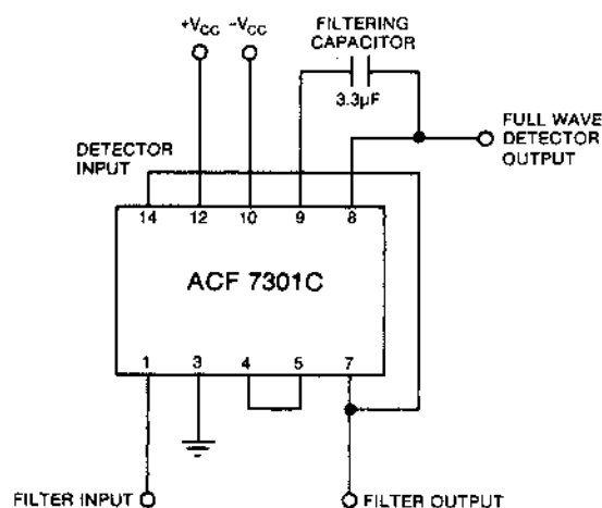
Fig.2 TYPICAL APPLICATION
