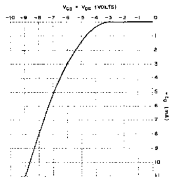
TURN-ON CHARACTERISTICS
