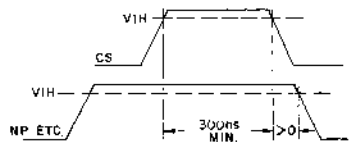
Fig.15c CS
