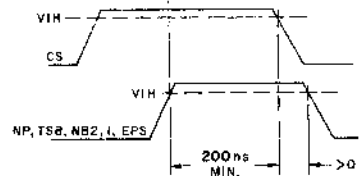
Fig.37a CS
