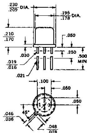
Bottom view
