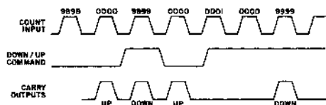
CARRY OPERATION
