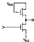
Fig.4 TYPICAL INPUT
