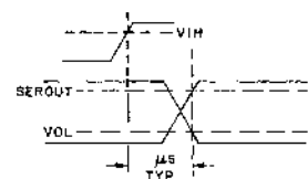
Fig.38 SEROUT
