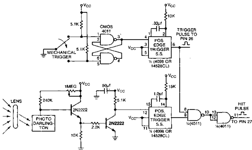
Fig.7 RIFLE INTERFACE
