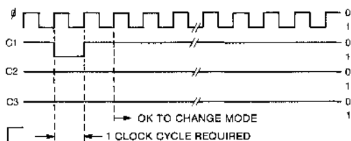
Fig.2 READ
