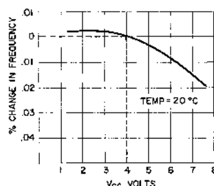
Fig.2. OSCILLATOR CHARACTERISTICS
