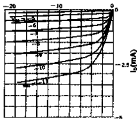
DRAIN CHARACTERISTICS AT 25°C V_{GS} (VOLTS)
