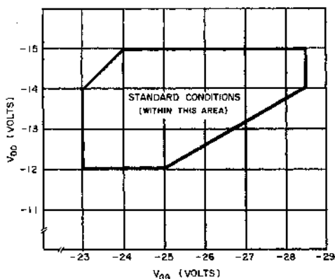
Fig.1 OPERATING VOLTAGES
