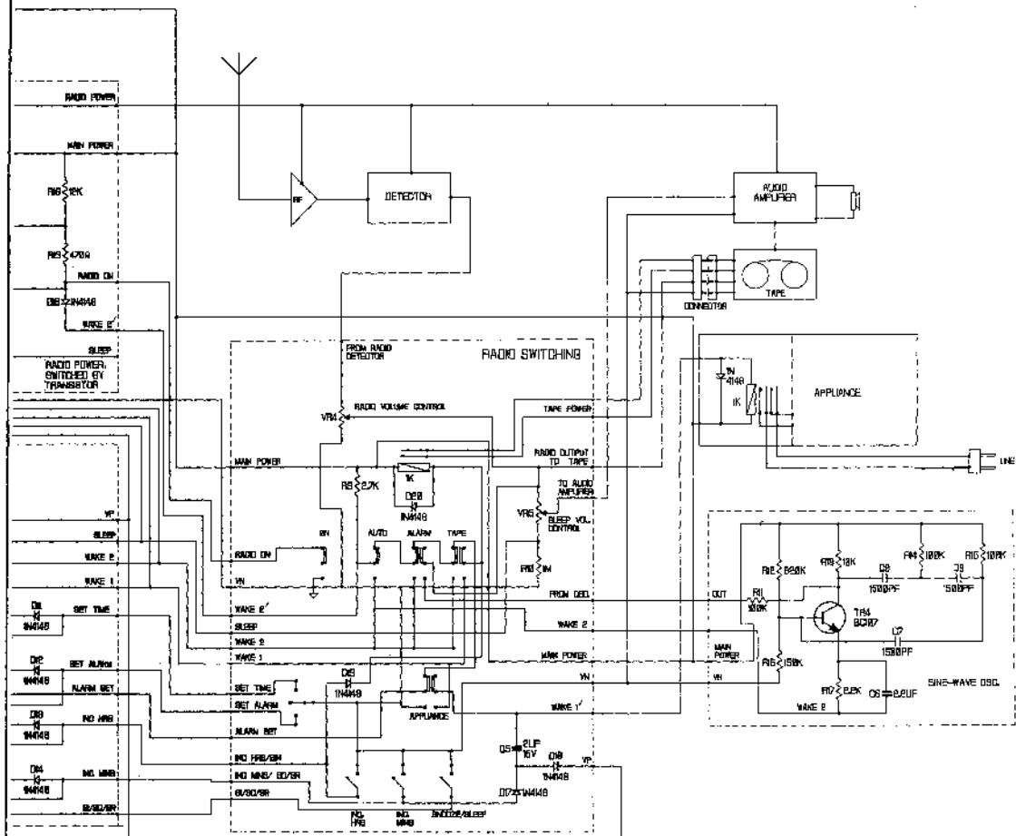
Fig.22(b) TYPICAL "FULL-FEATURE" CLOCK RADIO CIRCUITRY
