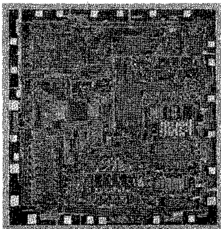
Microphoto of AY-3-8500 TV Game chip.
