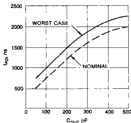
Fig. 46 RD1-RD8, PE, FE, OR, TBMT, DAV
