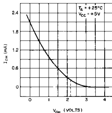
Fig.6 OUTPUT SOURCE CURRENT VS. OUTPUT VOLTAGE
