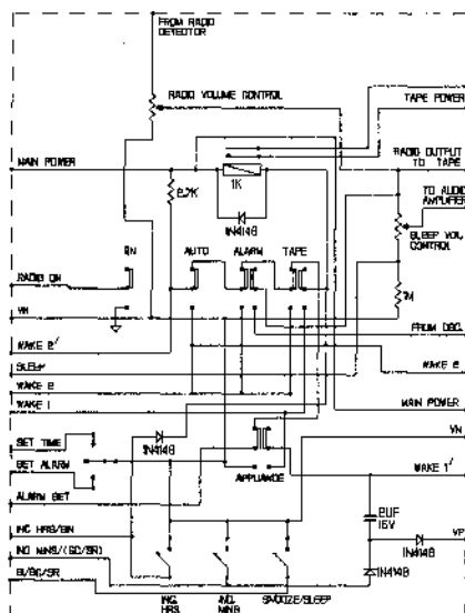
Fig.14 RADIO SWITCHING
