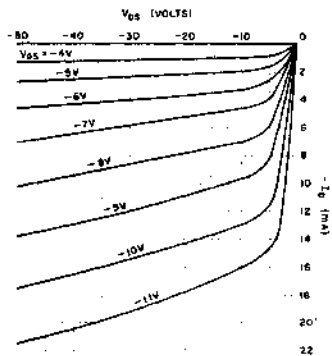
TRANSFER CHARACTERISTICS
