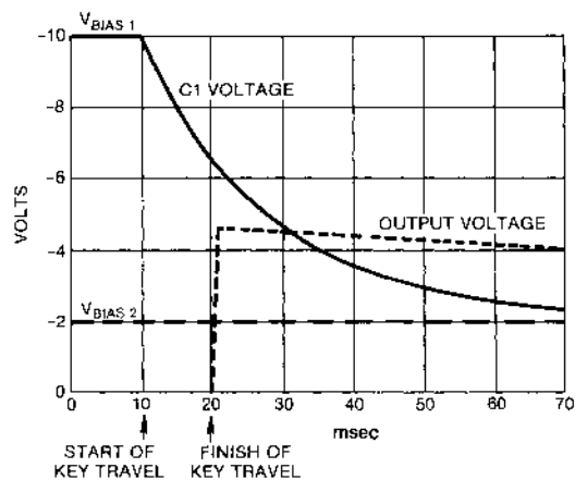
Fig.3 KEY VELOCITY WAVEFORMS
