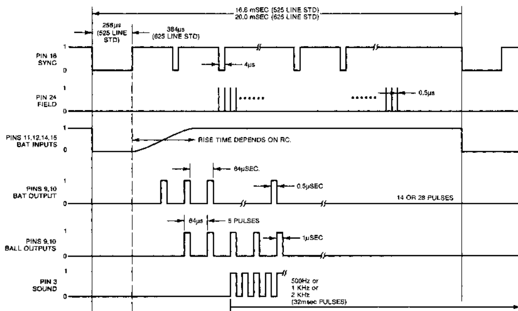
Fig. 11 TIMING DIAGRAM
