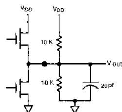
BUFFER OUTPUT TEST LOAD
