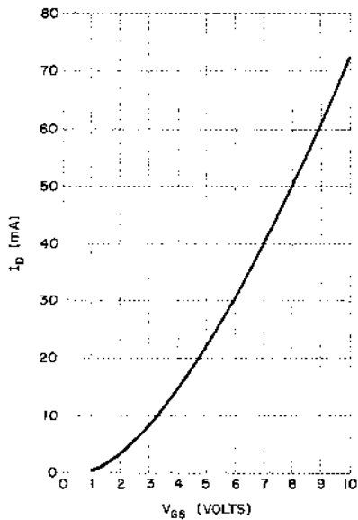
DRAIN CURRENT vs GATE VOLTAGE TRANSFER CHARACTERISTICS
