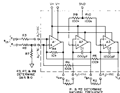
Fig. 2 TRIAD CONFIGURATION
