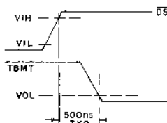
Fig.18 TBMT TURN-OFF
