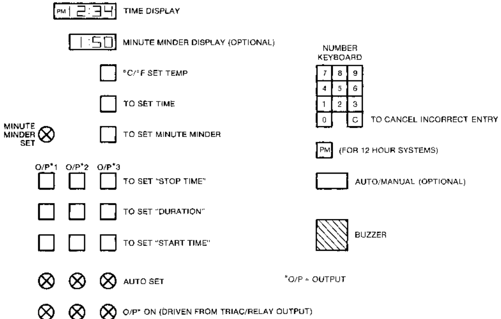
Fig. 2 TYPICAL AY-5-1251 CONTROLS FOR FULL KEYBOARD COOKER TIME
