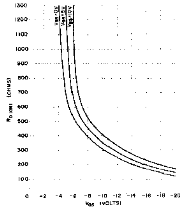
DRAIN TO SOURCE RESISTANCE vs. GATE VOLTAGE
