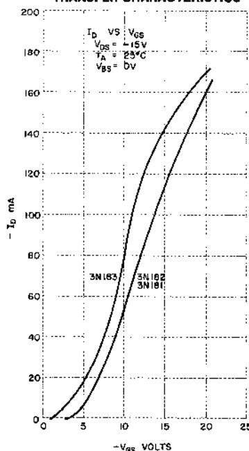
DRAIN CURRENT vs GATE VOLTAGE TRANSFER CHARACTERISTICS
