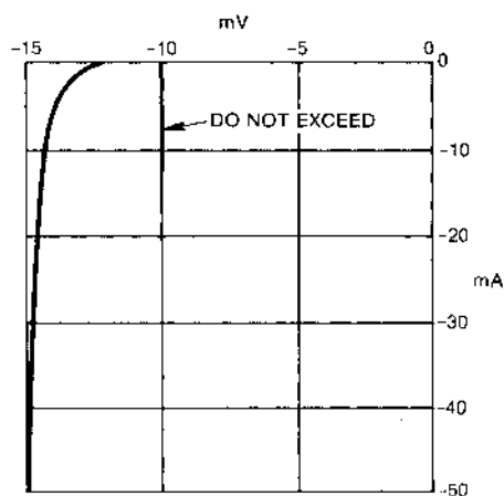
Fig.2 REVERSE BREAKDOWN
