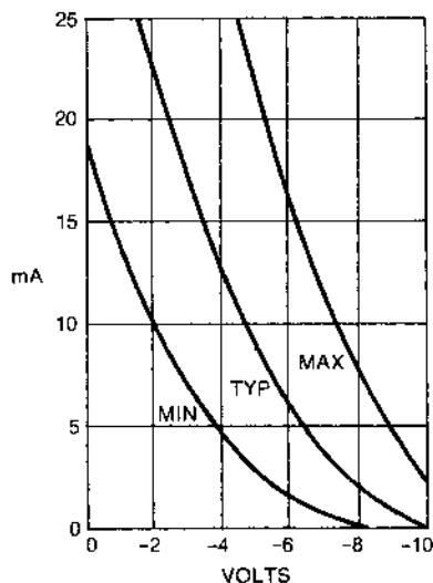
Fig.2 OUTPUT CHARACTERISTICS
