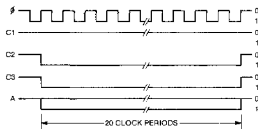
Fig.1 ACCEPT ADDRESS *
