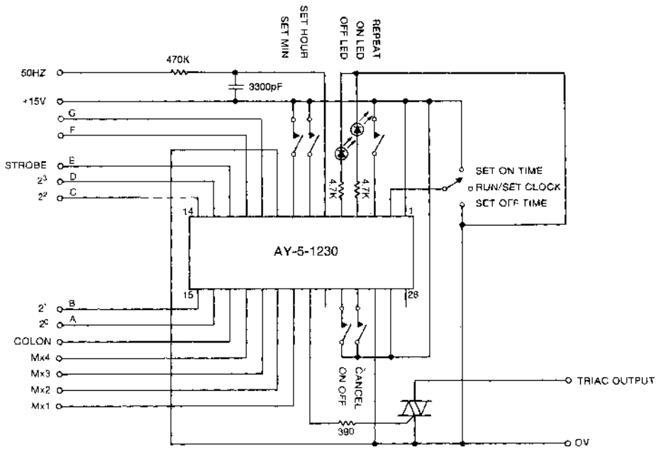
Fig.1 AY-5-1230 CONNECTION DIAGRAM
