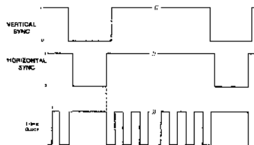
Fig.1 INPUT WAVEFORMS
