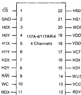
22-LEAD PDIP
