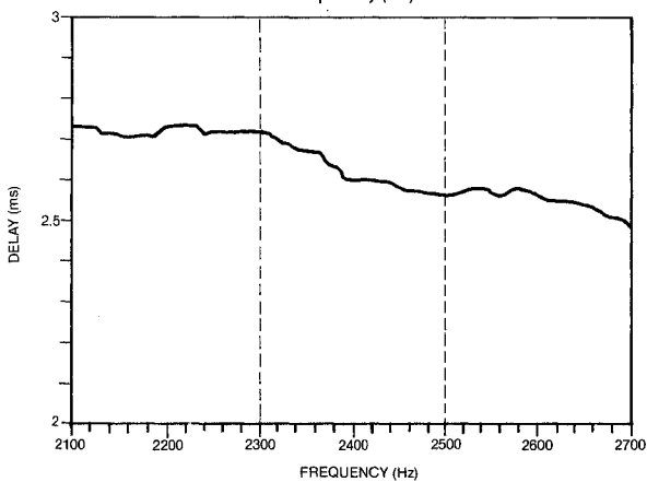
HIGH BAND Group Delay (ms)
