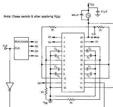
Fig. 3 — Dynamic power dissipation test circuit for SSI 22101
