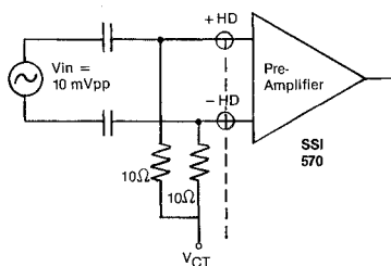
FIGURE 1 Preamplifier Characteristics
