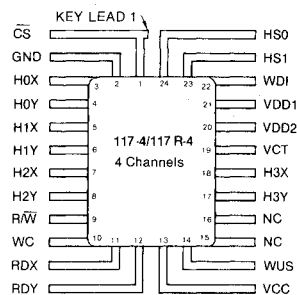
24-LEAD FLAT PACK
