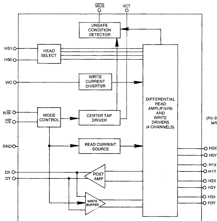
Block Diagram
