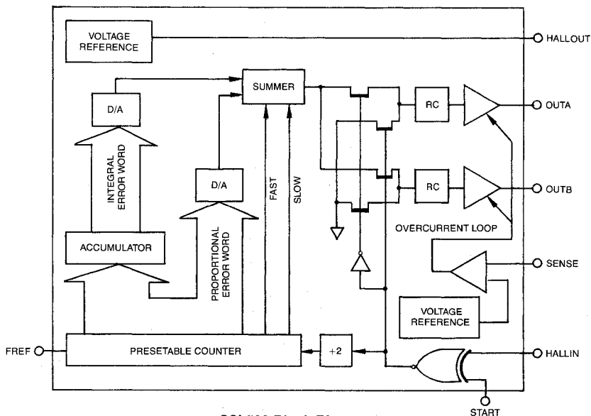
SSI 590 Block Diagram
