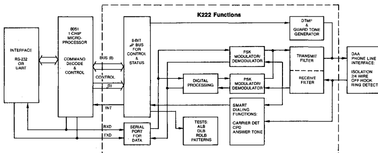
SSI K222 Block Diagram
