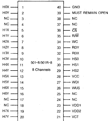
40-LEAD CDIP, PDIP
