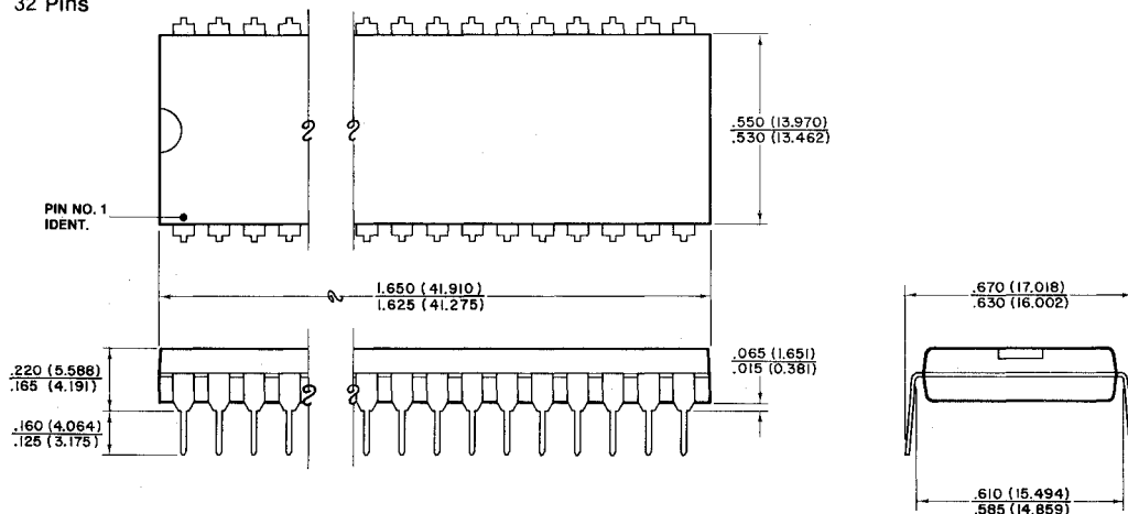
PLASTIC DIP 32 Pins
