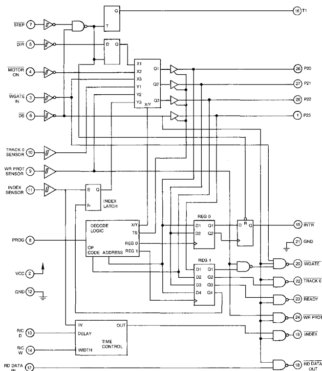
SSI 580 Block Diagram
