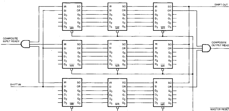
Figure 6. 192x12 FIFO.
