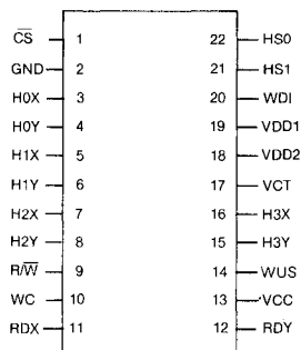
22-LEAD PDIP
