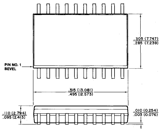
SOL 20 Leads
