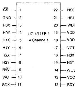
22-LEAD PDIP
