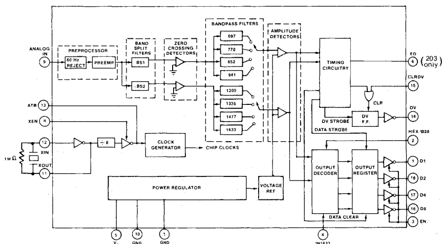
SSI 202/203 Block Diagram
