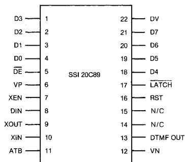
Pin Out (Top View)
