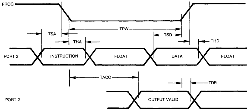
Figure 2. Timing Diagram
