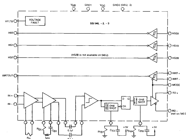
SS1 540-1, -2, -3 Block Diagram
