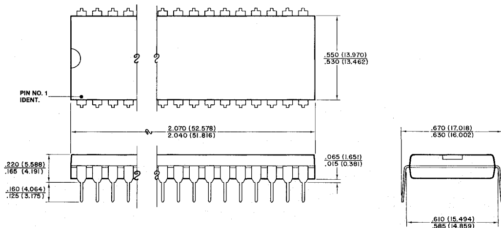
PLASTIC DIP 40 Pins
