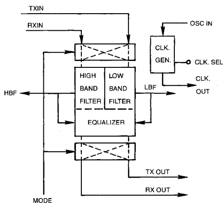
SSI 3522 Block Diagram
