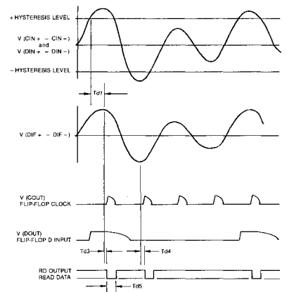
Fig. 2: Timing Diagram
