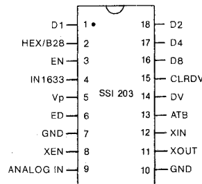
Pin Out (Top View)
