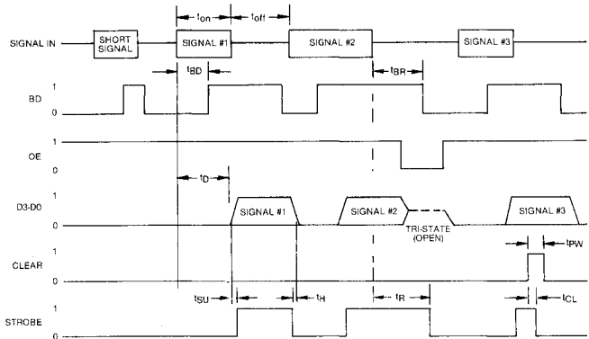
Figure 1. Timing Diagram
