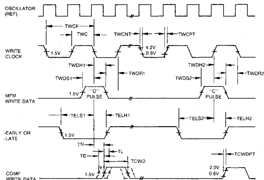
Figure 2 - Write Precompensation Waveforms
