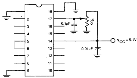
Fig.4 - Test circuit for impedance measurement.
