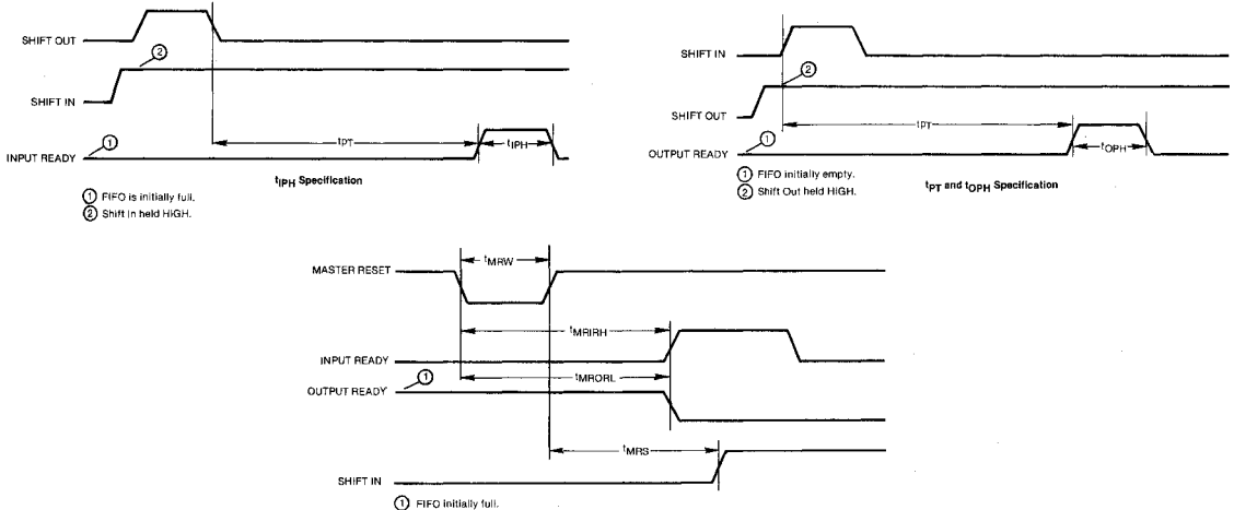
Master Reset Timing Figure 4. Timing Waveforms
