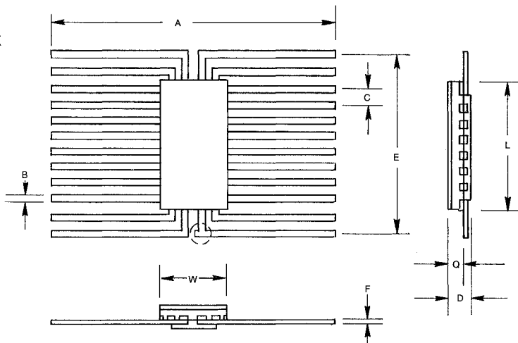
FLAT PACK 24 Leads
