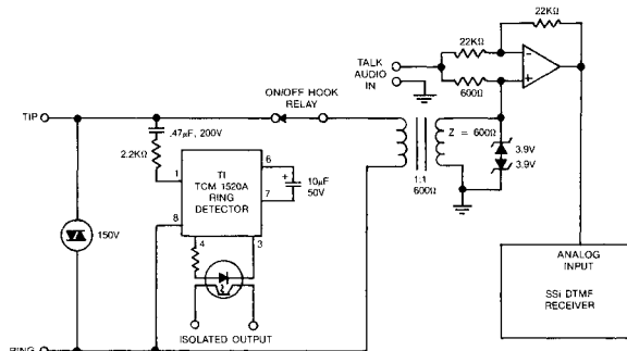
Figure 6. Full Featured Phone Line Interface
