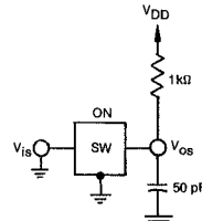
Propagation delay time test circuit and waveforms (data-in to signal output, switch Turn-ON to high or low level).
