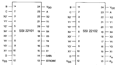
Pin Out (Top View)
