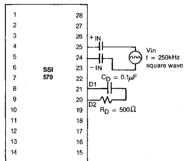
FIGURE 3 Postamplifier Threshold Differential Input Voltage
