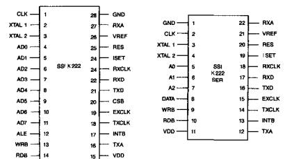
Preliminary Pin Configuration
