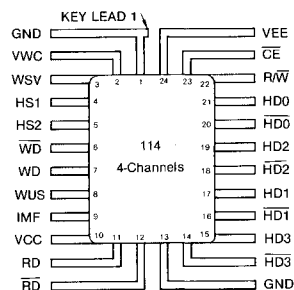
SSI 114 Pin Out
