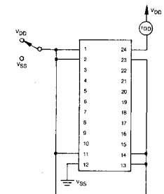
Fig. 1 — Quiescent current test circuit
