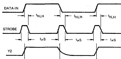
Fig. 10 — Strobe to Data-In hold time t_H for SSI 22101.
