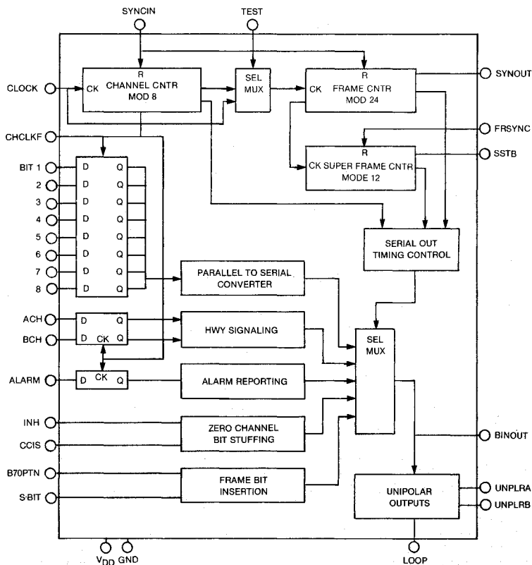
SSI 80C50 Block Diagram
