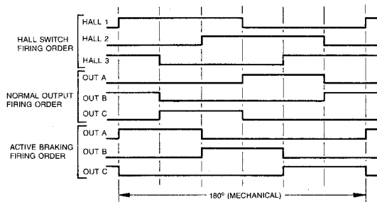
Figure 1: — Hall Switch/Driver Timing Relationship
