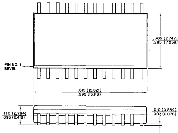
SOL 24 Leads
