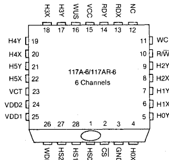
28-LEAD QUAD
