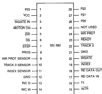
28-LEAD PDIP (Top View)
