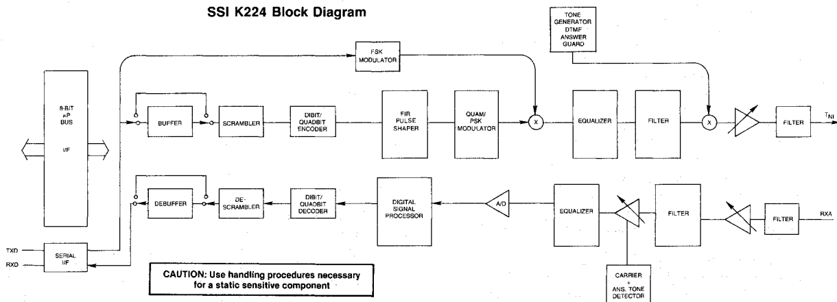
SSI K224 Block Diagram
