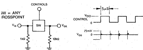
Fig. 11 — Test circuit and waveforms for crosstalk (control input to signal output).
