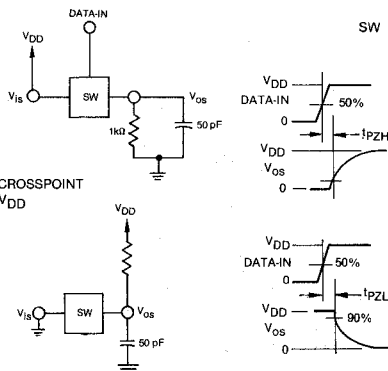
Fig. 7 — Propagation delay time test circuit and waveforms (data-in to signal output, switch Turn-ON to high or low level).
