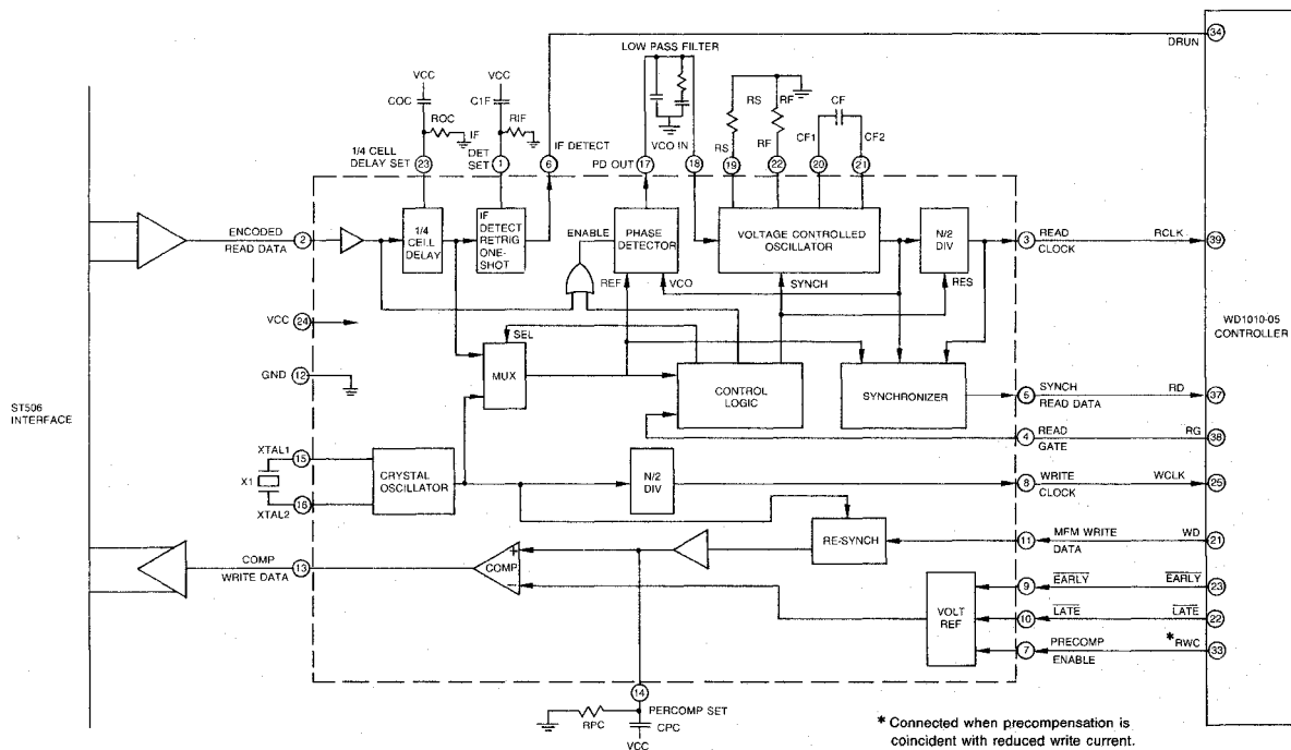
Fig. 3 — Typical System Connections
