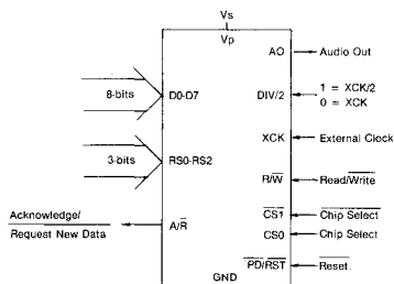
Signal Diagram
