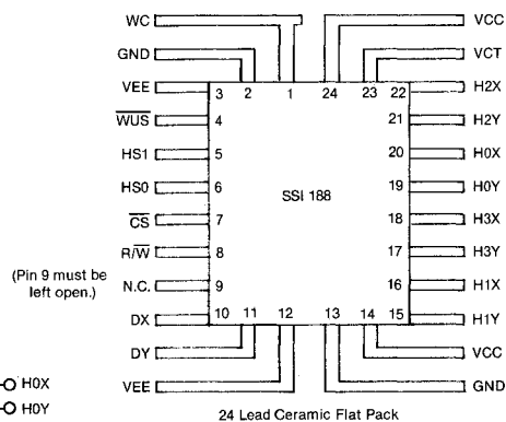
Pin Out (Top View)
