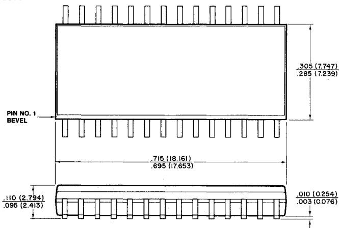
SOL 28 Leads
