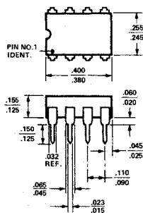
Plastic Dip 8-Pins
