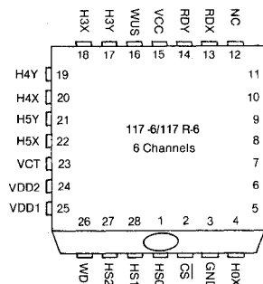
28-LEAD PLCC (QUAD)
