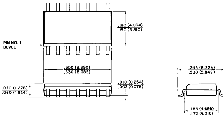
SON 14 Leads
