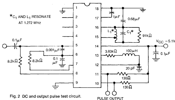
Fig. 2 DC and output pulse test circuit.
