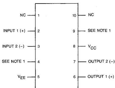
Flat Pack
