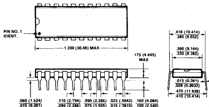
PLASTIC DIP 22 Pins
