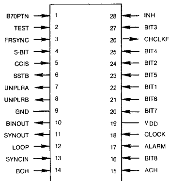
Pin Out (Top View)
