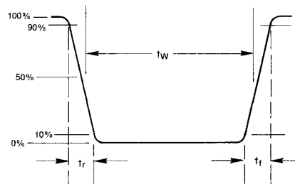
Fig.6 · Output pulse waveform.
