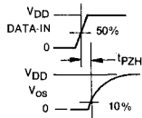
Propagation delay time test circuit and waveforms (data-in to signal output, switch Turn-ON to high or low level).
