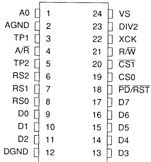
24-Pin DIP
